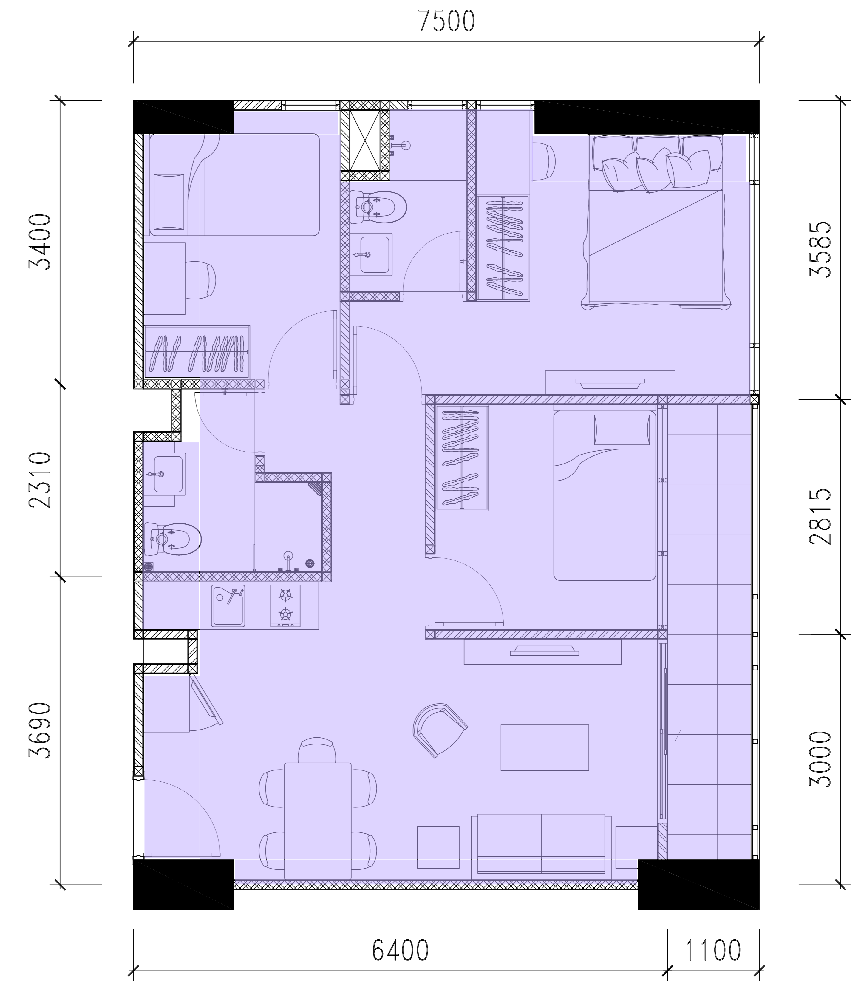
UNIT 3BA Semi Gross = 89,81 m2
