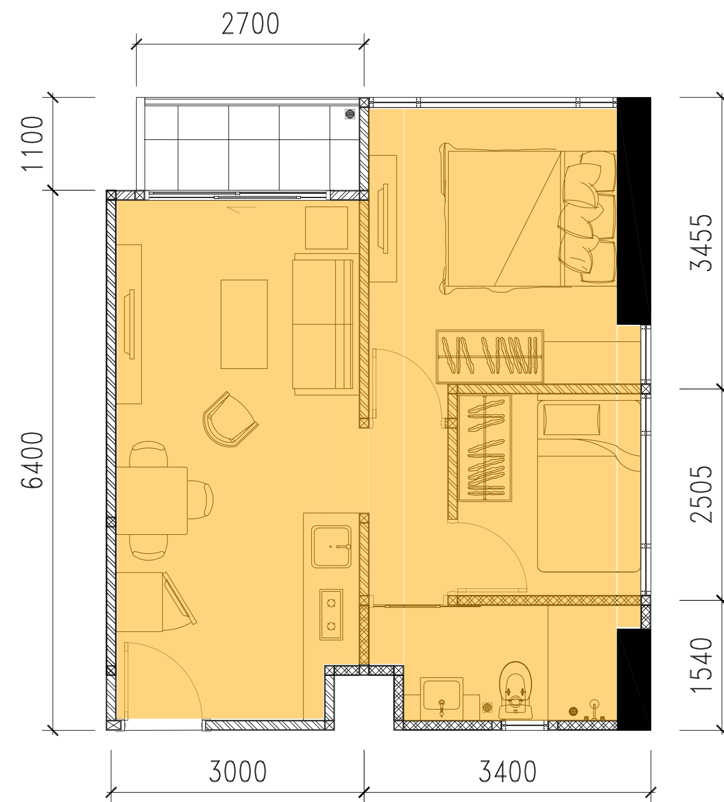
UNIT 2BA Semi Gross = 60,73 m2
