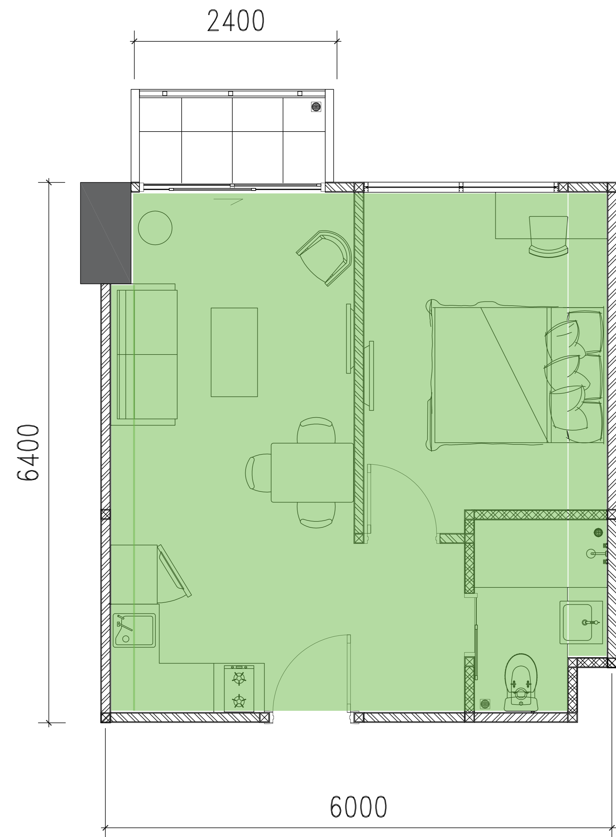
UNIT 1BA Semi Gross = 52,28 m2
